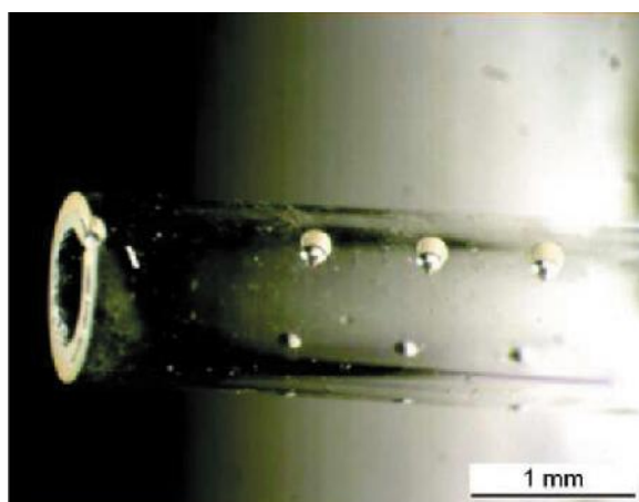
Figure 1 – Hollow fiber with holes
