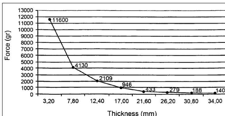
Figure 2 – Thickness of the wall as a function of the magnetic force
